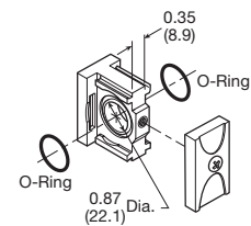
Body Connector
